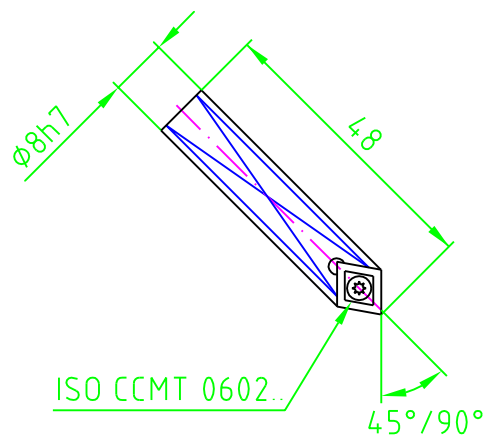
Insert holder 45°/90°
