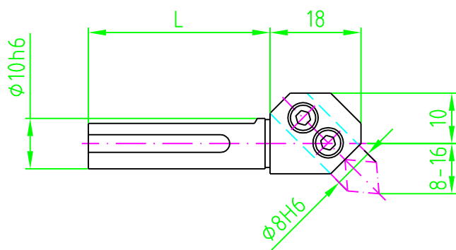
Insert holder 90°
