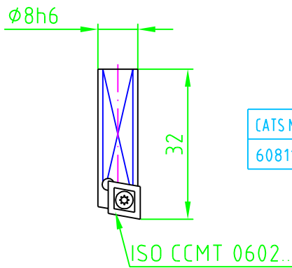
Insert holder 90°
