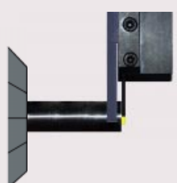
The chuck jaws are unclamped and the bar is pulled out into the new cutting position
