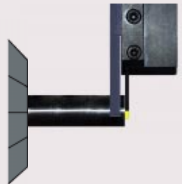
The chuck jaws are unclamped and the bar is pulled out into the new cutting position
