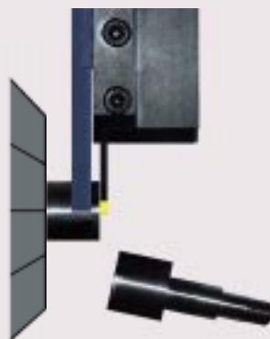
After cut-off the spindle is stopped
